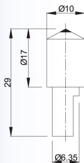
Rockwell Indenter 0.2 R 120^\circ
